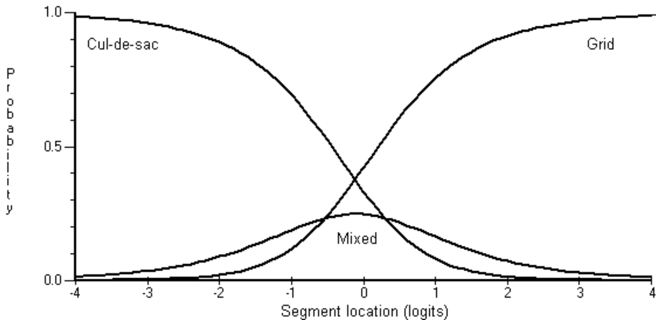
Figure 1 Category Characteristic Curve showing dysfunctional scoring model for street pattern.
