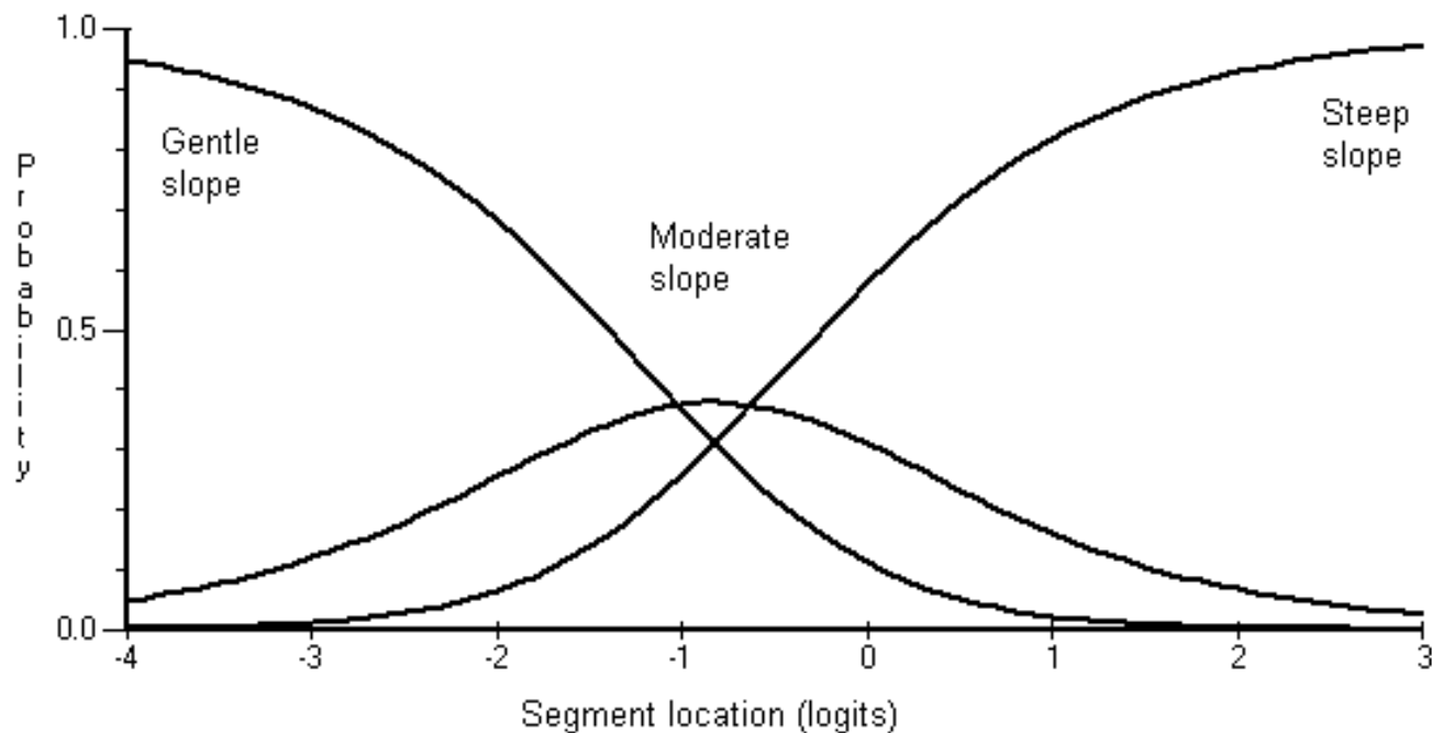
Figure 2 Category Characteristic Curve showing normal functioning scoring model for path/road slope.
