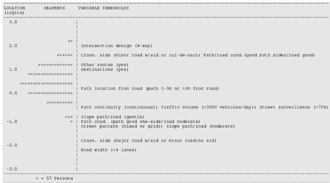
Figure 3 Segment and item threshold location on the functional environment scale.
