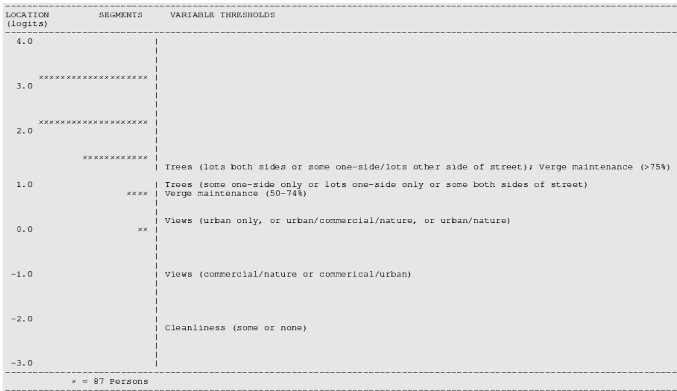
Figure 4 Segment and item threshold locations on the aesthetic environment scale.
